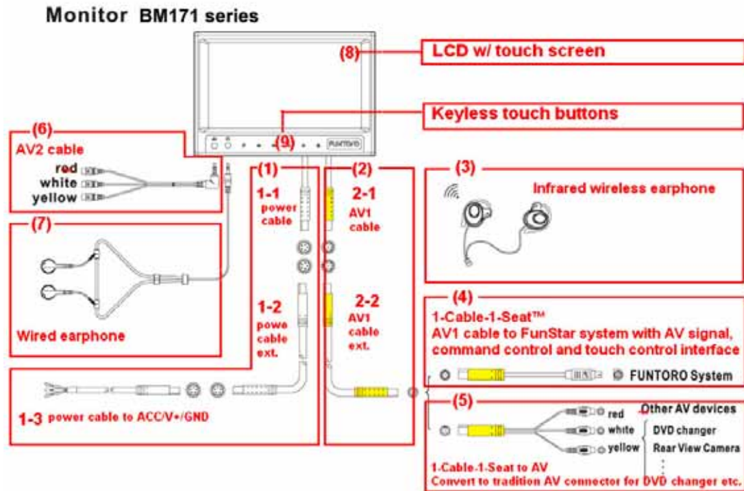
Figure 3 Product Installation kits
